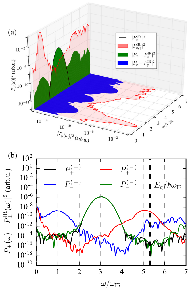
FIG. 2. The spectral analysis of the polarization response for F_{\text{IR}} = 1 \text{ V/\AA} and the zero pump-probe delay. (a) The x and y components of the IR-only response \mathbf{P}^{\text{IR}} (pale red), the UV-only response \mathbf{P}^{\text{UV}} (black curve), and the polarization induced by both pulses after subtracting the IR-only response: \mathbf{P} - \mathbf{P}^{\text{IR}} (the green and blue areas). All the curves are plotted on the same scale. (b) The decomposition of \mathbf{P} - \mathbf{P}^{\text{IR}} into the left- and right-rotating components induced by the left- and right-rotating components of the UV pulse (see the text for further details). The vertical black dashed line shows the position of the band edge.
